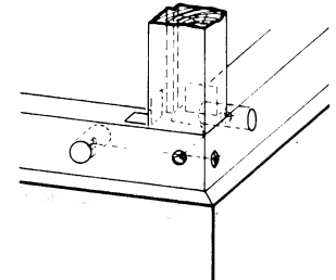
5 Sill corner reanchored with cap screws
